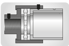
FRTC Full recessed thrust collar.
